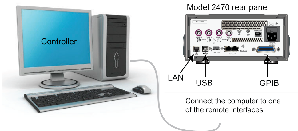
Figure 20: Model 2470 remote interface connections
