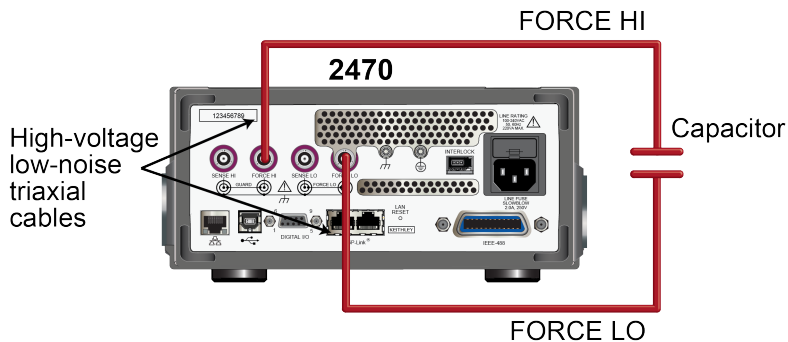
Figure 22: Rear-panel connections for the leakage current test
