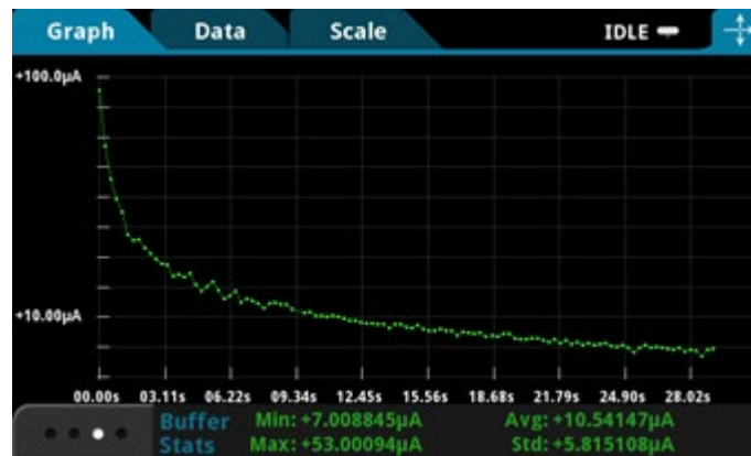
Figure 24: Front panel graph of leakage current measurement
