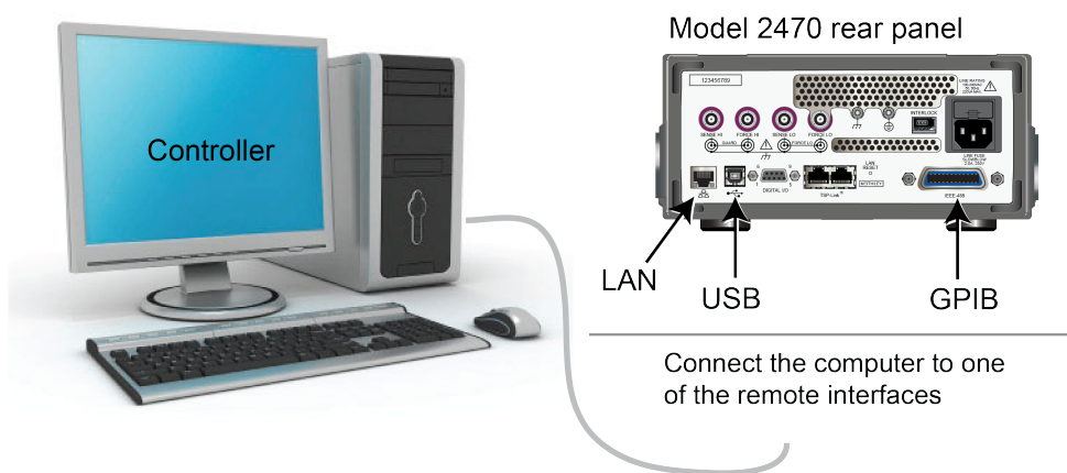
Figure 28: Model 2470 remote interface connections
