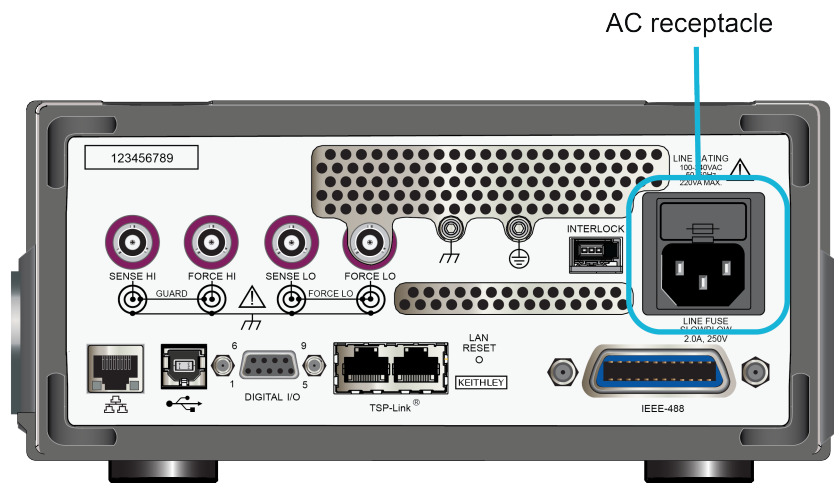
Figure 1: Model 2470 AC receptacle on rear panel
