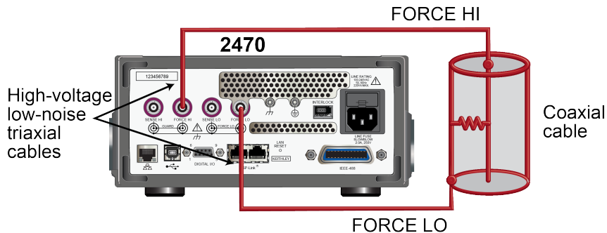
Figure 23: Rear-panel connections insulation resistance test
