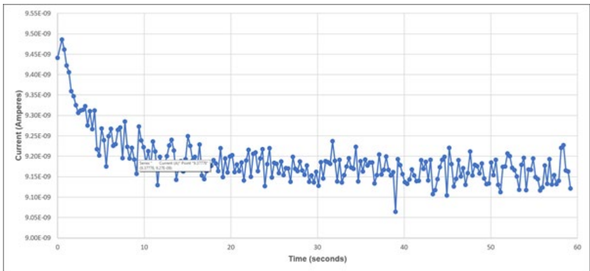
Figure 35: Drain leakage current graph
