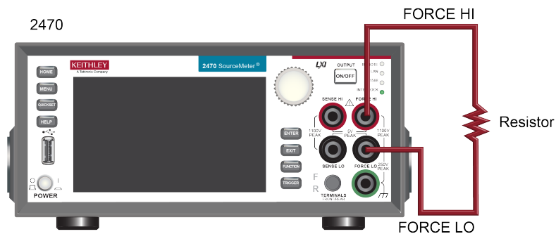
Figure 19: 2470 2-wire front-panel connections
