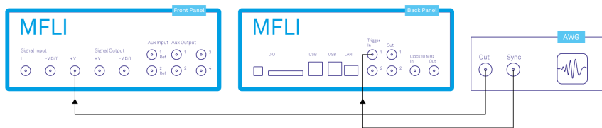
Figure 4.59: MFLI connections to an external arbitrary waveform generator
