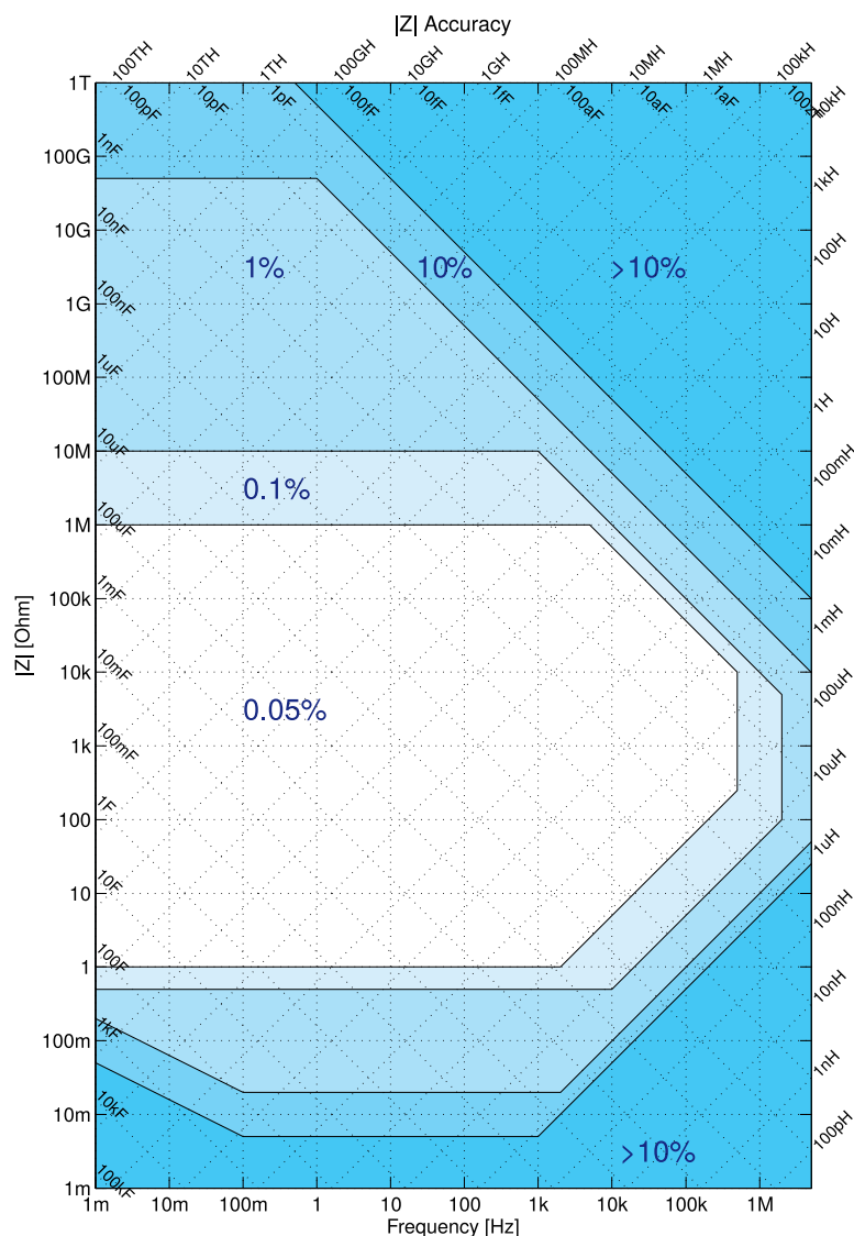
Figure 4.39: Impedance Accuracy chart
