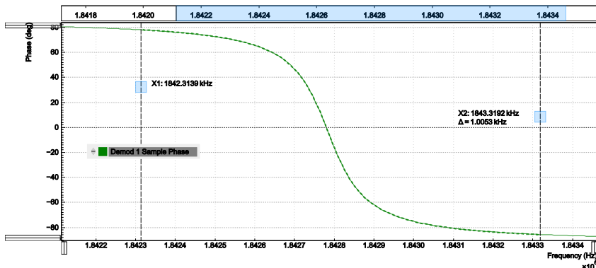
Figure 4.51: Phase of the resonator's frequency response measured with the LabOne Sweeper. Solid line are measurement data, dashed line is a fit to the response function of an LCR circuit model using the resonance fitting tool.
