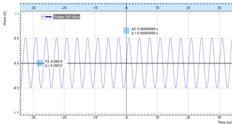
Figure 4.19: LabOne Scope showing the raw signal generated by the MFLI
