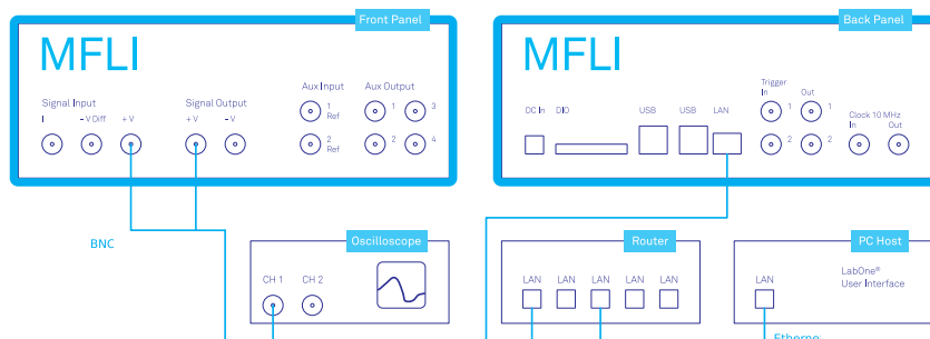
Figure 4.18: Setup for the Simple Loop Tutorial (LAN connection shown)
