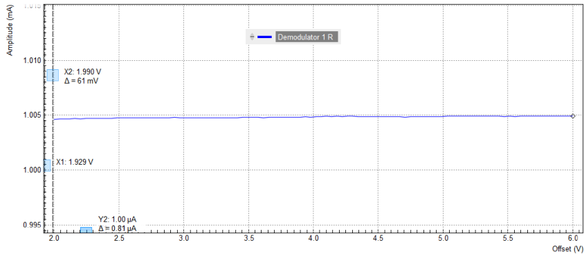
Figure 4.31: Gate voltage dependence of the MOSFET source current measured with the LabOne Sweeper in a four-terminal setup
