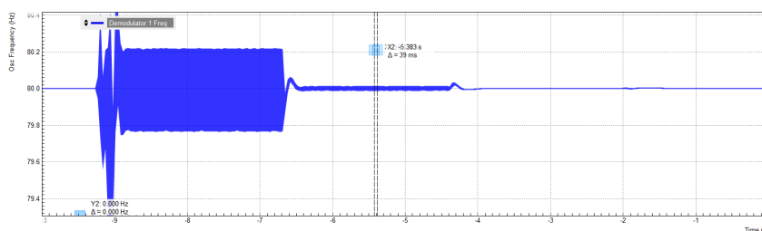
Figure 4.25: Frequency of the internal oscillator over time with stepwise automatic bandwidth adjustment
