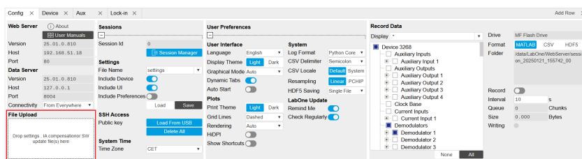
Figure 2.33: Config Tab showing drop zone for software update
