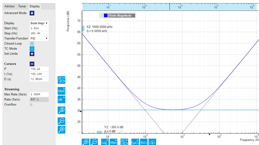
Figure 4.55: Graphical setting of the PID parameters using the cursors. The three cursor lines with negative, zero, and positive slope correspond to the frequency dependence of the P, I, and D parts of the controller, respectively.
