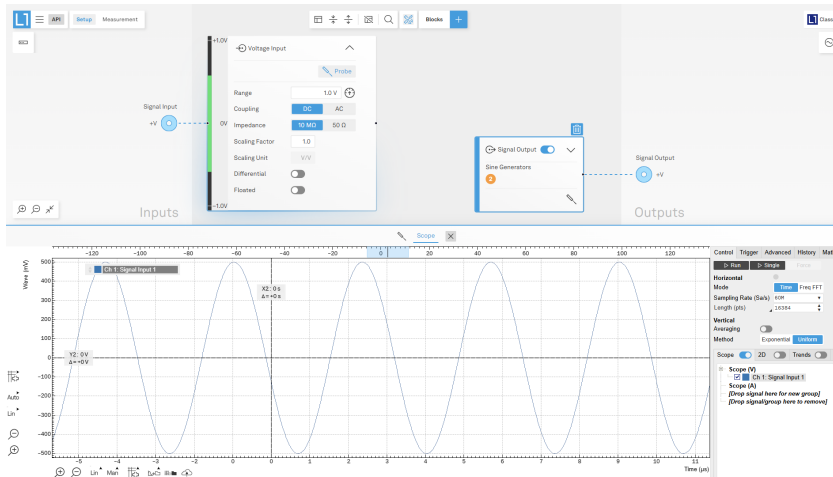
Figure 4.5: Observing the input signal using the probe feature. The input sine wave is visible in the scope window.
