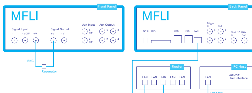
Figure 4.53: PID connection with MF instrument
