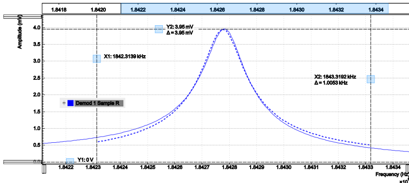
Figure 4.50: Amplitude of the resonator's frequency response measured with the LabOne Sweeper. Solid line are measurement data, dashed line is a fit to the response function of an LCR circuit model using the resonance fitting tool.
