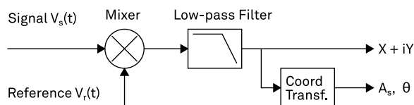
Figure 6.2: Mixing and low-pass filtering performed by the lock-in amplifier
