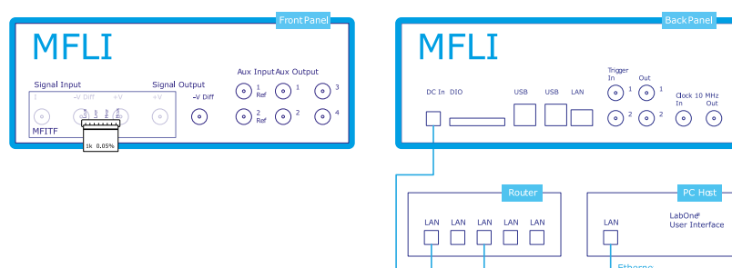
Figure 4.33: Setup for the Impedance Measurement Tutorial
