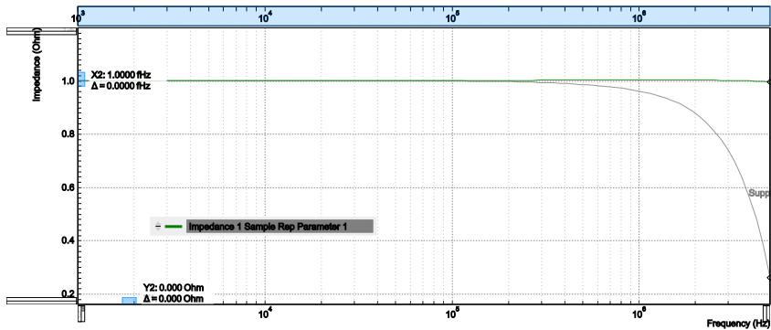
Figure 4.47: LabOne Sweeper showing the resistance of a 1 \Omega DUT measured with compensation (green) and without (grey)
