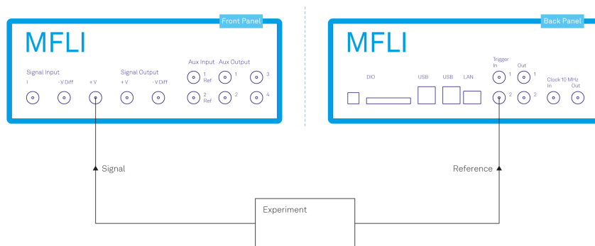
Figure 4.9: Setup for the external reference measurement.
