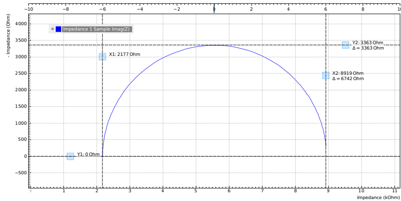
Figure 4.43: Nyquist plot of an R-R-C sample
