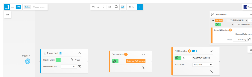
Figure 4.14: Frequency lock of an internal oscillator to an external reference signal is established.
