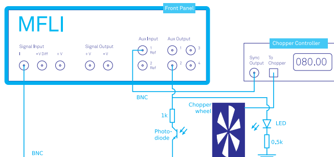
Figure 4.22: Setup for the external reference measurement with optical chopper, LED, and photo diode.
