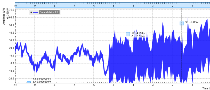
Figure 4.21: LabOne User Interface Plotter displaying demodulator results while changing the filter bandwidth from 10 Hz to 1 kHz
