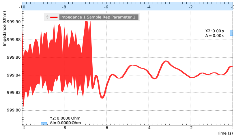
Figure 4.38: LabOne Plotter showing a resistance measurement over time. Changing the filter setting manually leads to a change in noise.
