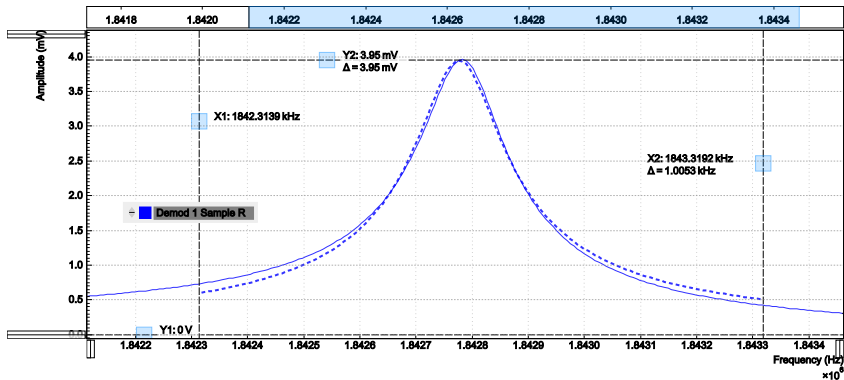
Figure 4.54: Amplitude of the resonator’s frequency response measured with the LabOne Sweeper. Solid line are measurement data, dashed line is a fit to the response function of an LCR circuit model using the resonance fitting tool.
