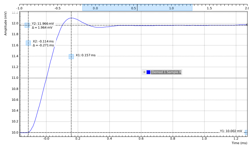
Figure 4.57: Closed-loop step response measured with the Data Acquisition tool
