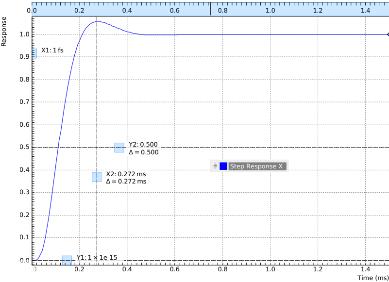
Figure 4.56: Closed-loop step response simulated with the PID Advisor
