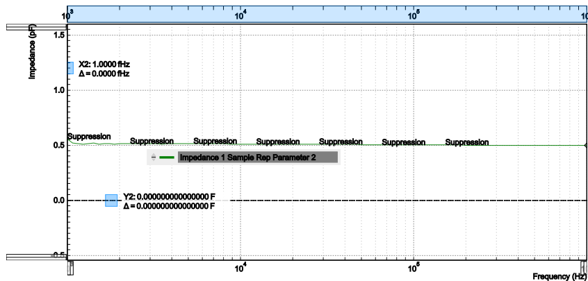
Figure 4.42: Replacement circuit capacitance of a 1 M \Omega through-hole device measured with the LabOne Sweeper
