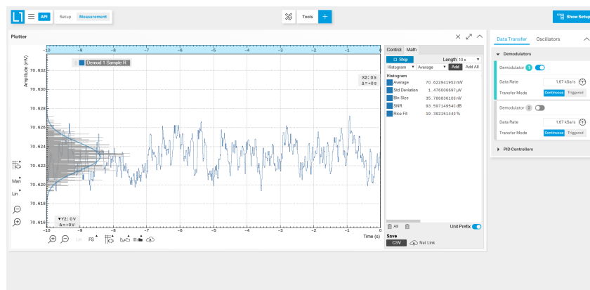
Figure 4.16: Plotter tool in the Measurement workspace, displaying the time trace of demodulated amplitude.
