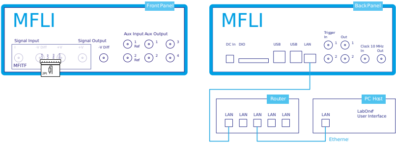
Figure 4.40: Setup for the Impedance Measurement Tutorial. The measured device is a resistor soldered onto one of the through-hole DUT carriers that come with the MFITF.
