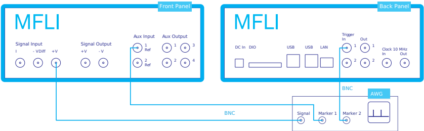
Figure 4.58: Setup for the imaging tutorial with MF Instrument
