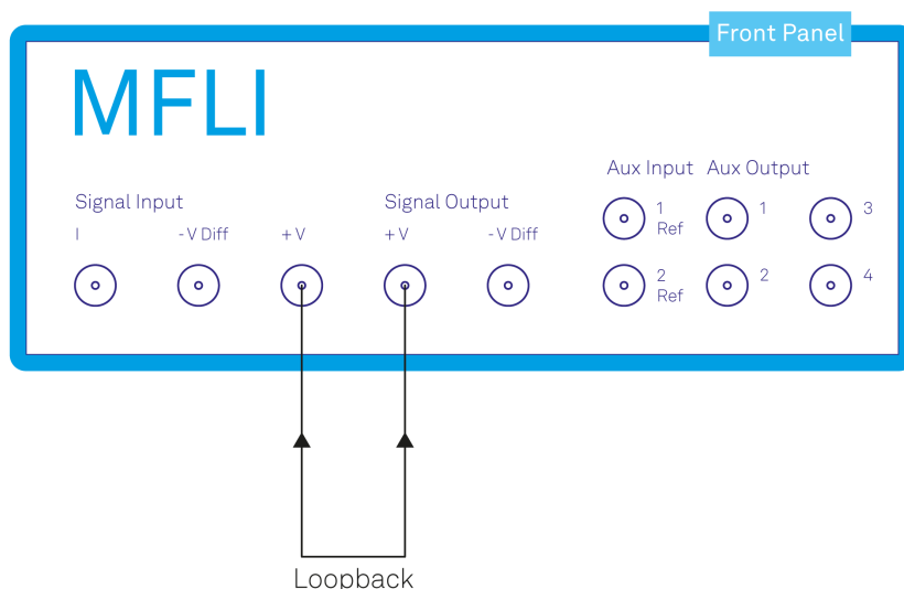
Figure 4.1: Setup for the Simple Loop tutorial.
