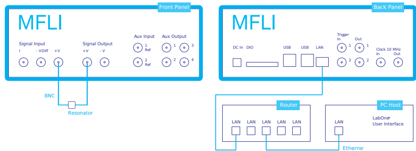
Figure 4.49: PLL connection with MF Instrument
