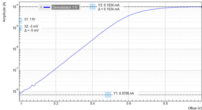
Figure 4.30: Gate voltage dependence of the MOSFET source current measured with the LabOne Sweeper
