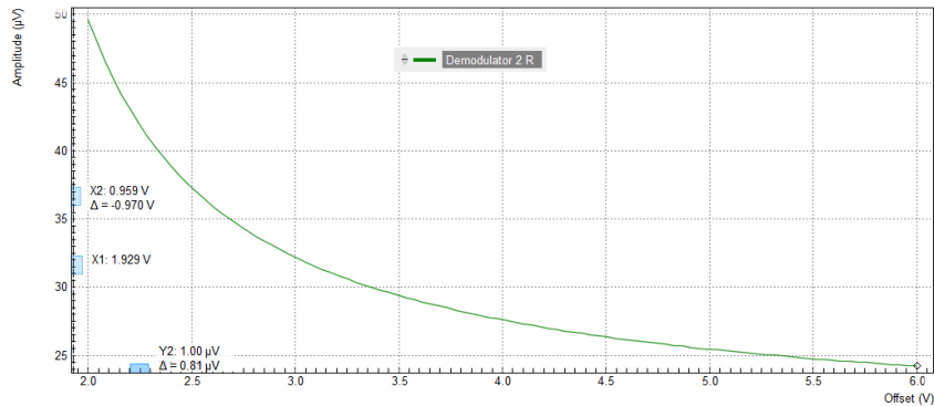
Figure 4.32: Gate voltage dependence of the MOSFET drain-source voltage measured with the LabOne Sweeper in a four-terminal setup
