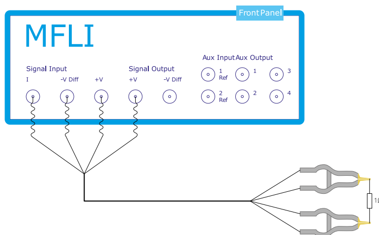
Figure 4.45: Setup for the Impedance Compensation Tutorial
