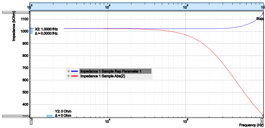
Figure 4.41: Absolute Impedance |Z|
