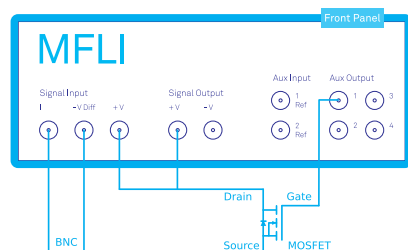
Figure 4.29: Setup for the MOSFET measurements.
